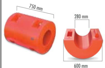
M03528 120 LT Buoyancy: 108 kg
