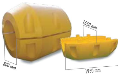
M03580 2580 LT Buoyancy: 2320 kg
