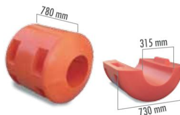
M03532 176 LT Buoyancy: 160 kg
