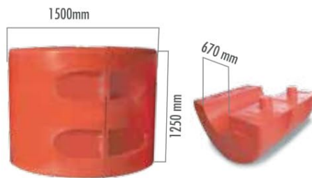
M03567 1700 LT Buoyancy: 1530 kg
