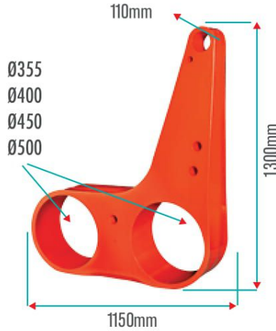
ORANJ BRAKET ORANGE BRACKET
