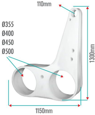
FOSFORLU BRAKET PHOTOLUMINESCENT BRACKET
